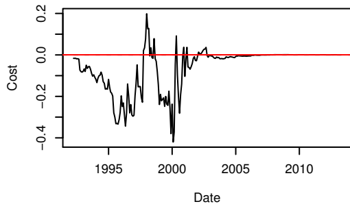
Hedging Error
