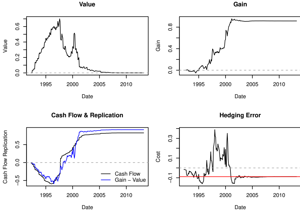
Figure 4: Sparse model replication strategy for US VC funds of vintage 1992. Here the variables introduced in section 2.1 are used as follows: Value is V , Gain is G , Cash Flow is A , and Hedging Error is calculated as A - (G - V) = Y - G .
