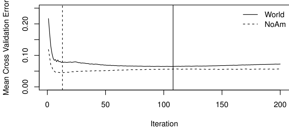
Figure 2: Leave-One-Vintage-Out cross validation results for \lambda = 2\% .
