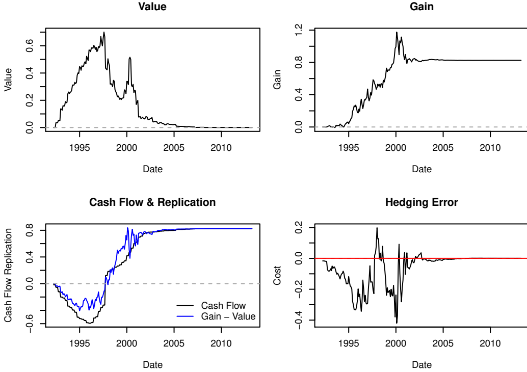
Figure 1: Simple ex-post replication strategy for US VC funds of vintage 1992. Here the variables introduced in section 2.1 are used as follows: Value is V , Gain is G , Cash Flow is A , and Hedging Error is calculated as A - (G - V) = Y - G .
