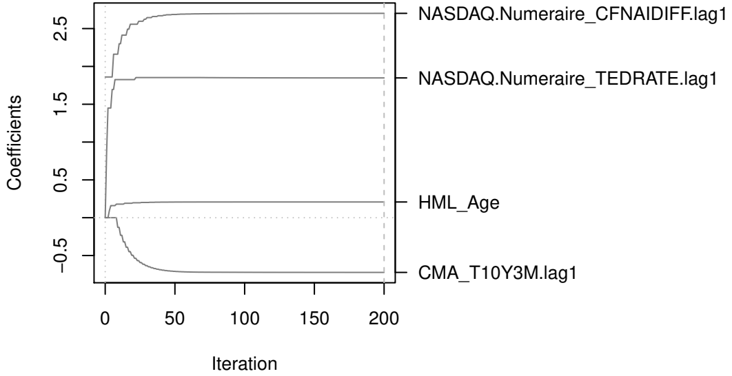
Figure 3: Sparse model coefficients based on stability selection for \lambda^* = 2\% and S^* = \text{World} .
